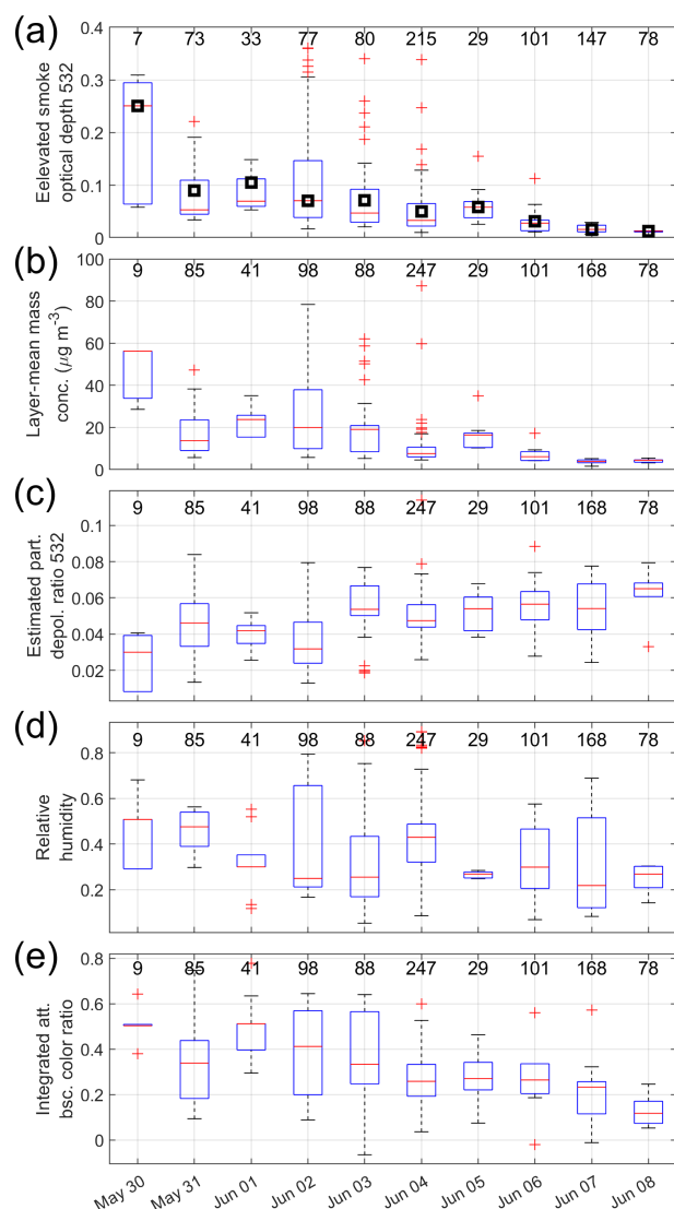
Figure 4. Statistical properties of smoke layers originating from the Alberta plume event on 29 May 2019. CALIPSO Level-2 5 km ALayer products were used. In case of overlapping layers in the vertical, 5 km APro products were used to calculate the AODs. Used layer numbers (or profile numbers in panel a ) in each boxplot are given on the top. AODs of the smoke layers used in Fig. 5 are shown as black squares in panel ( a ).
