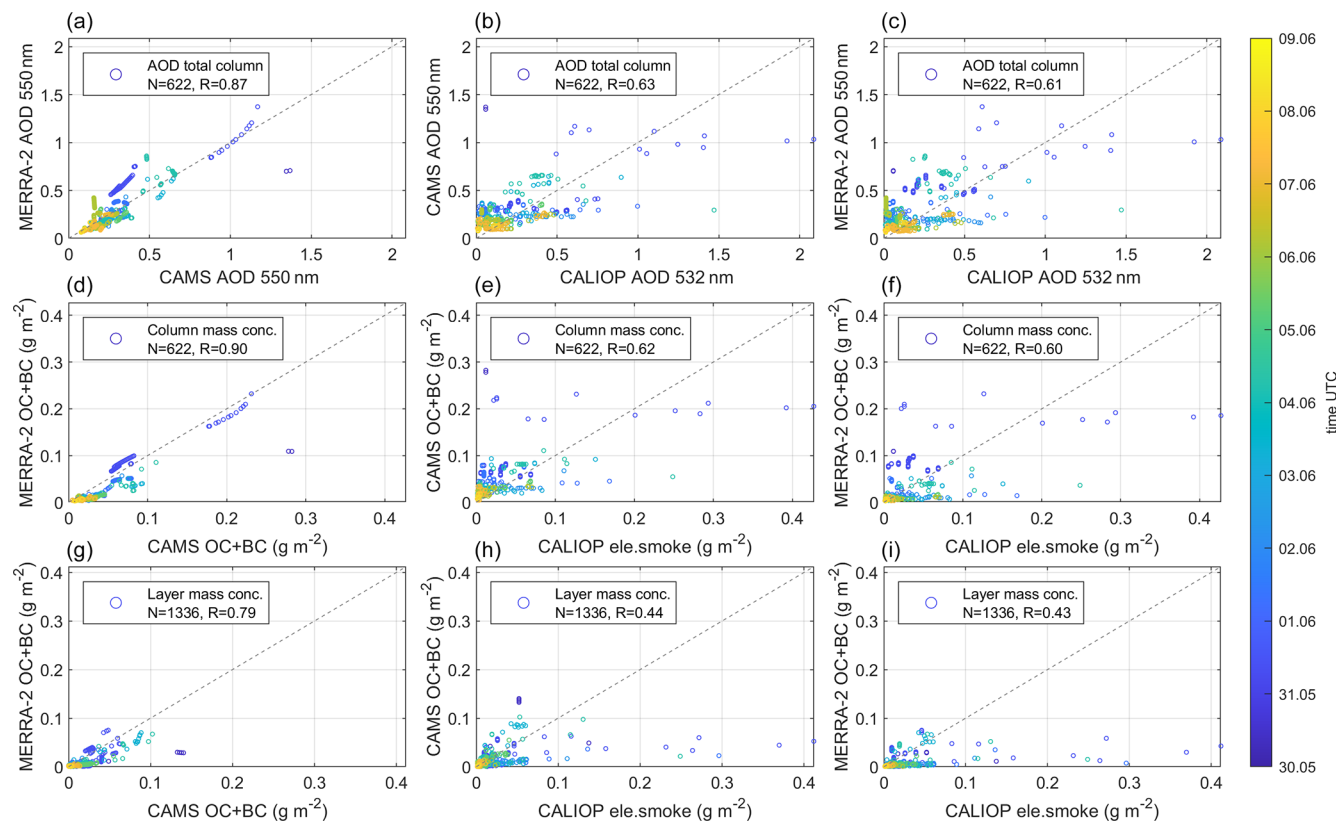
Figure 6. Comparison of observed and simulated products for locations where CALIPSO detected smoke layers: (a–c) total column AOD (tropospheric AODs from CALIPSO); (d–f) column mass concentration of black carbon (BC) and organic carbon (OC) of CAMS and MERRA-2, and summed layer mass concentration of CALIPSO elevated smoke layers; (g–i) layer mass concentrations of CALIPSO elevated smoke layers and layer mass concentrations (three times the depth of the CALIPSO layers) of BC and OC of CAMS and MERRA-2.
