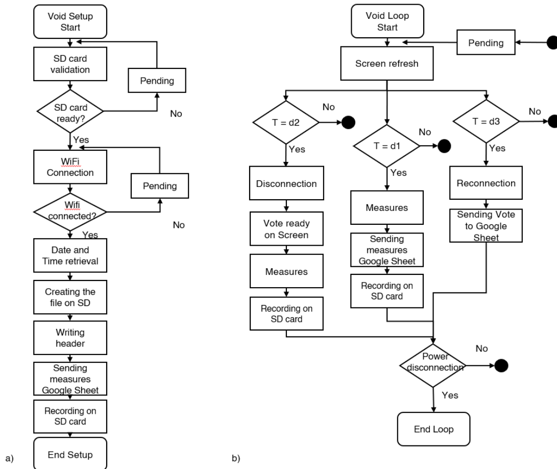
Figure 1. Program flowchart: a) Void Setup, b) Void Loop
