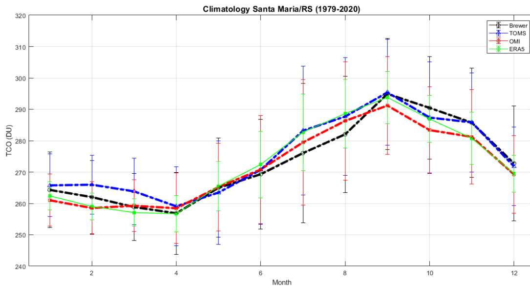
Figure 2. Monthly climatology for TOC in SM with satellite data TOMS (blue) and OMI (red) and ERA5 reanalysis (green) between 1979-2020 and, ground-based data with Brewer spectrophotometer (black) at intervals 1992-2017.
