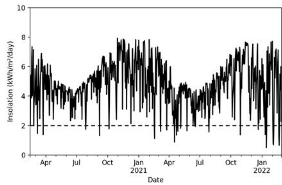
Fig. 4. Daily insolation received on a horizontal surface at the experimentation site in Mafate. The dashed line represents the threshold for considering a very low insolation level.
