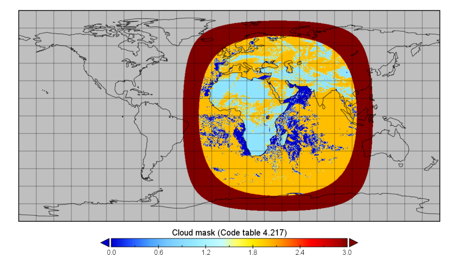
Fig 4: Cloud mask obtained from Meteosat
