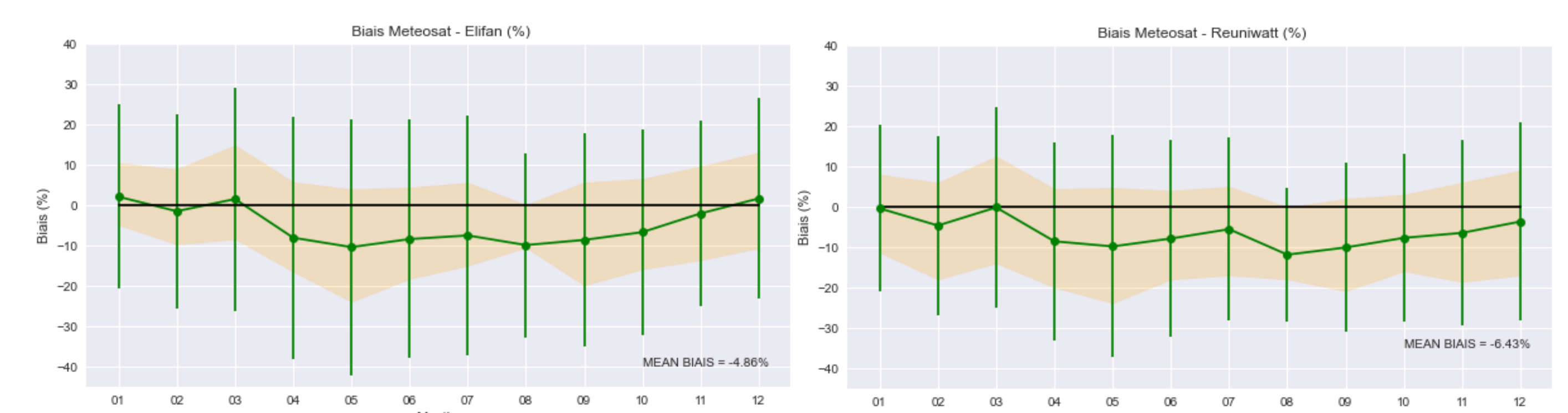
Fig 7: Bias of Cloud Fraction (Meteosat and Elifan / Reuniwatt) - St Denis - La Réunion
