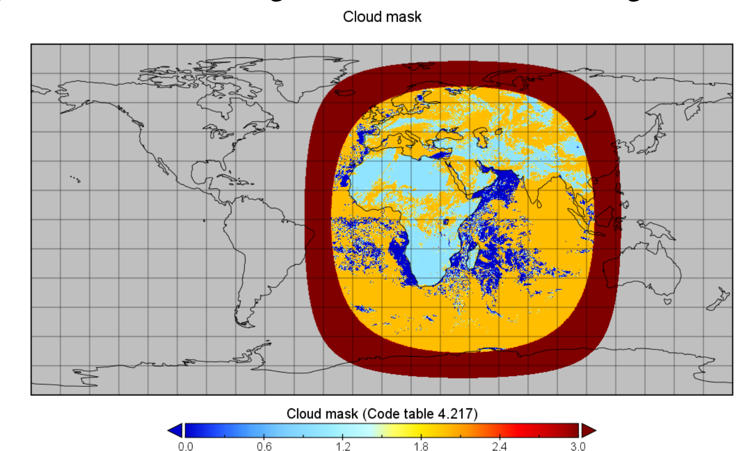
Fig 4: Cloud mask obtained from Meteosat
