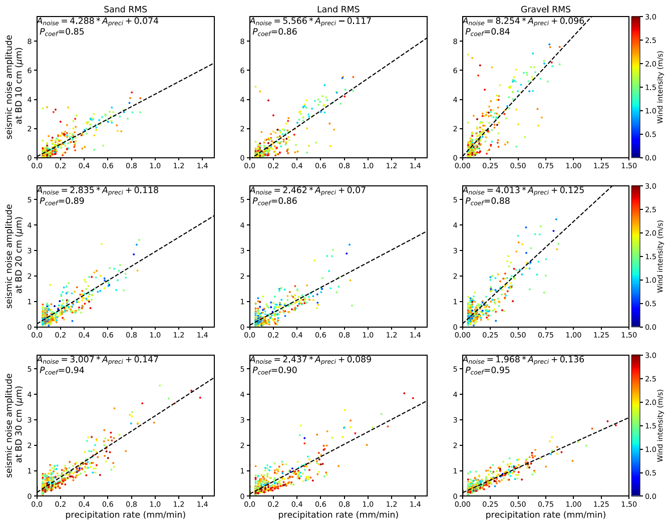
Figure 8. Scatter plot between the root mean square of the precipitation rate and seismic noise amplitude for sand (left column), andisol (middle) and gravel (right column); for the different burial depth 10 cm (top), 20 cm (center), and 30 cm (bottom). The transfer function between the two parameters, which correspond to the dashed black lines are presented at the top left corner, together with the corresponding Pearson coefficient ( P_{coef} ). The dots colors mark the wind intensity, as indicated on the right scale.
