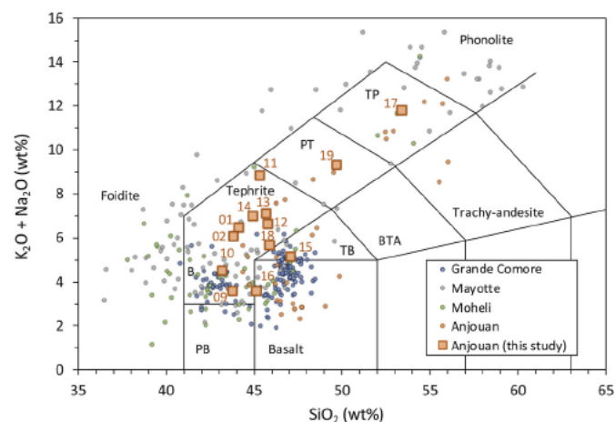
Fig. 3. The total alkali versus silica (TAS) diagram for rocks from the Comoros Islands. Data have been extracted from the Georoc database (see text for references). The large orange square symbols are for samples from this study, with the number above each corresponding to sample name. Samples from previous studies are shown with small circles with a given color for each island. Rock fields are from Le Bas et al. (1986). PB: Picro-basalt; B: Basanite; TB: Trachy-basalt; BTA: Basaltic trachy-andesite; PT: Phono-tephrite; TP: Tephri-phonolite.
