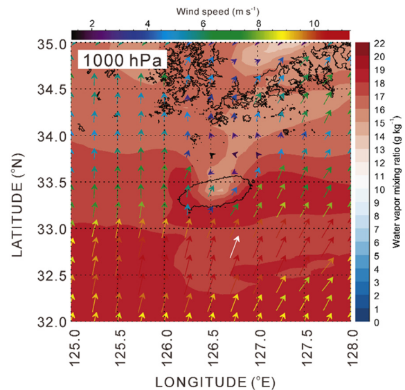
Fig. 4. Horizontal distribution of the water vapor mixing ratio (g kg -1 , shades) and wind (colored vectors) at the 1000-hPa level from MSM data at 1800 LST on July 04, 2012.
