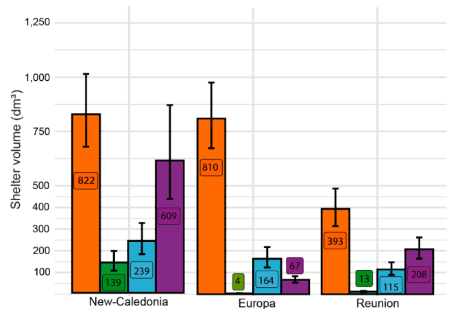
Fig. 7. Predictions for mean shelter volumes (bars) for each reefscape from planar area of colonies by growth forms: branching (orange), columnar (green), massive (blue) and tabular (purple) with lower and upper prediction intervals (black line). Prediction values are indicated for each bar.
