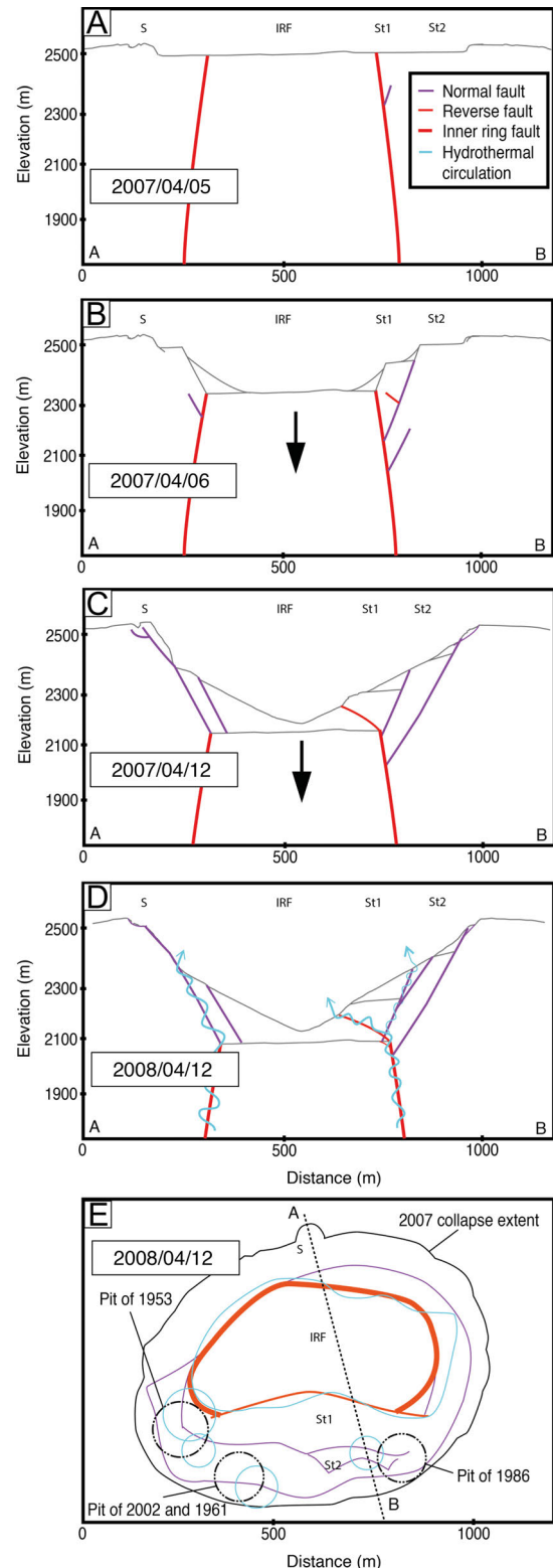
Figure 5: Interpretation of the temporal evolution of the April 2007 Dolomieu collapse on [A] April 5 th , [B] April 6 th , [C] April 12 th , 2007 and [D] April 12 th , 2008 after complete cessation of the collapse mechanism. [E] Related interpretative map as observed on April 12 th , 2008. S: Soufrière pit-crater, IRF: Inner Ring Fault, St1: Southern terrace 1, St2: Southern terrace 2.
