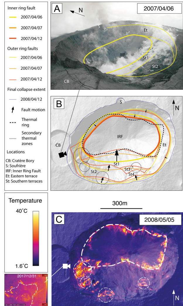
Figure 4: [A] Interpreted aerial photograph, courtesy of Peloton de Gendarmerie de Haute Montagne (PGHM), from the west of the Cratère Dolomieu on April 6 th , 2007. [B] Temporal and spatial evolution of the structures associated with the April 2007 Cratère Dolomieu collapse, as identified on [A] and on Figure 2. Note the progressive appearance of the terraces associated with development of the outer ring faults, with Et, St1 and St2 created between April 5 th and 6 th , St3 created between April 6 th and 7 th , and St4 created between April 7 th and 12 th . [C] Thermal orthoimage of the Cratère Dolomieu on May 5 th , 2008. The inset shows a thermal image of the caldera taken from the west on December 12 th , 2017.
