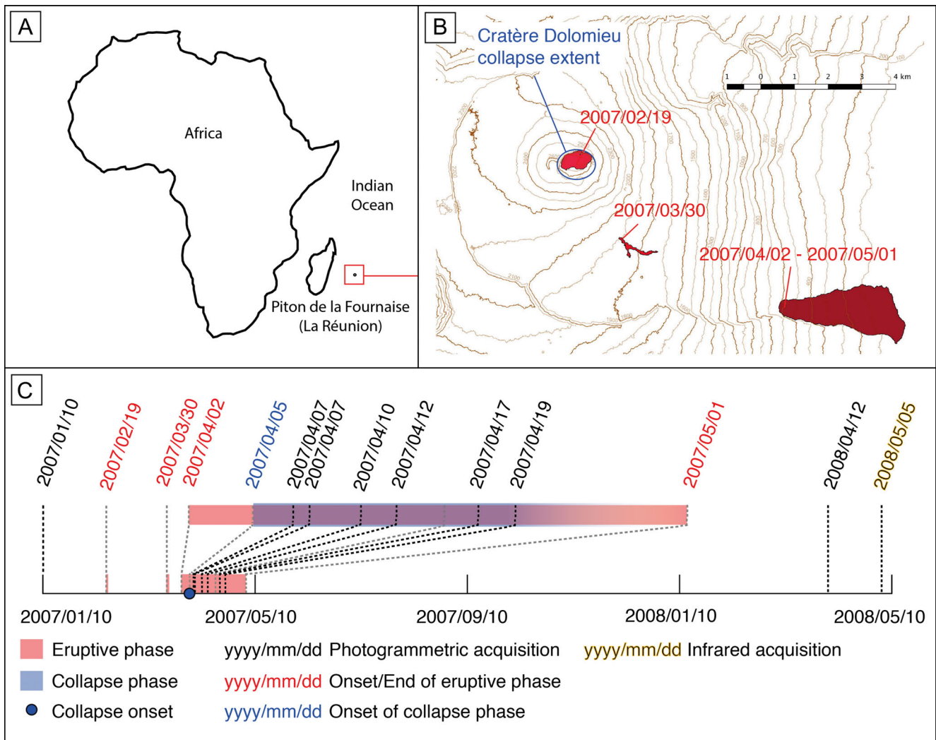
Figure 1: [A] Location of Piton de la Fournaise volcano. [B] Location of the April 2007 Cratère Dolomieu collapse and maps of the 2007 lava flows. [C] Timeline of the Piton de la Fournaise activity (eruptions and collapse) during the period of study. The dates of the aerial surveys used in this study are also reported.
