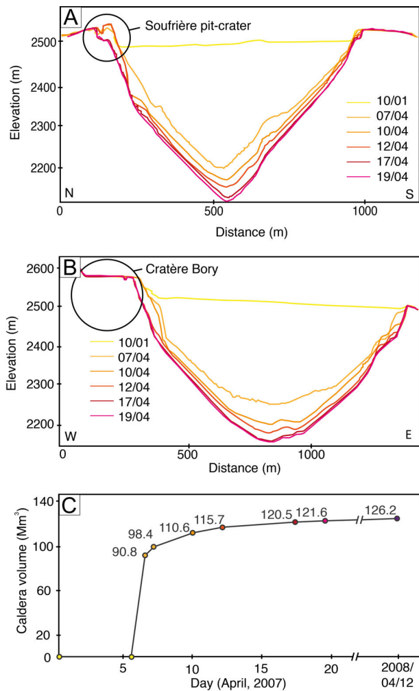
Figure 3: [A] N–S cross-sections of the successive DEMs made for 2007, with dates given in MM/DD format. [B] E–W cross-sections of the successive DEMs made for 2007. [C] Time series of the caldera volume evolution. See location of the cross-sections on Figure 2A.
