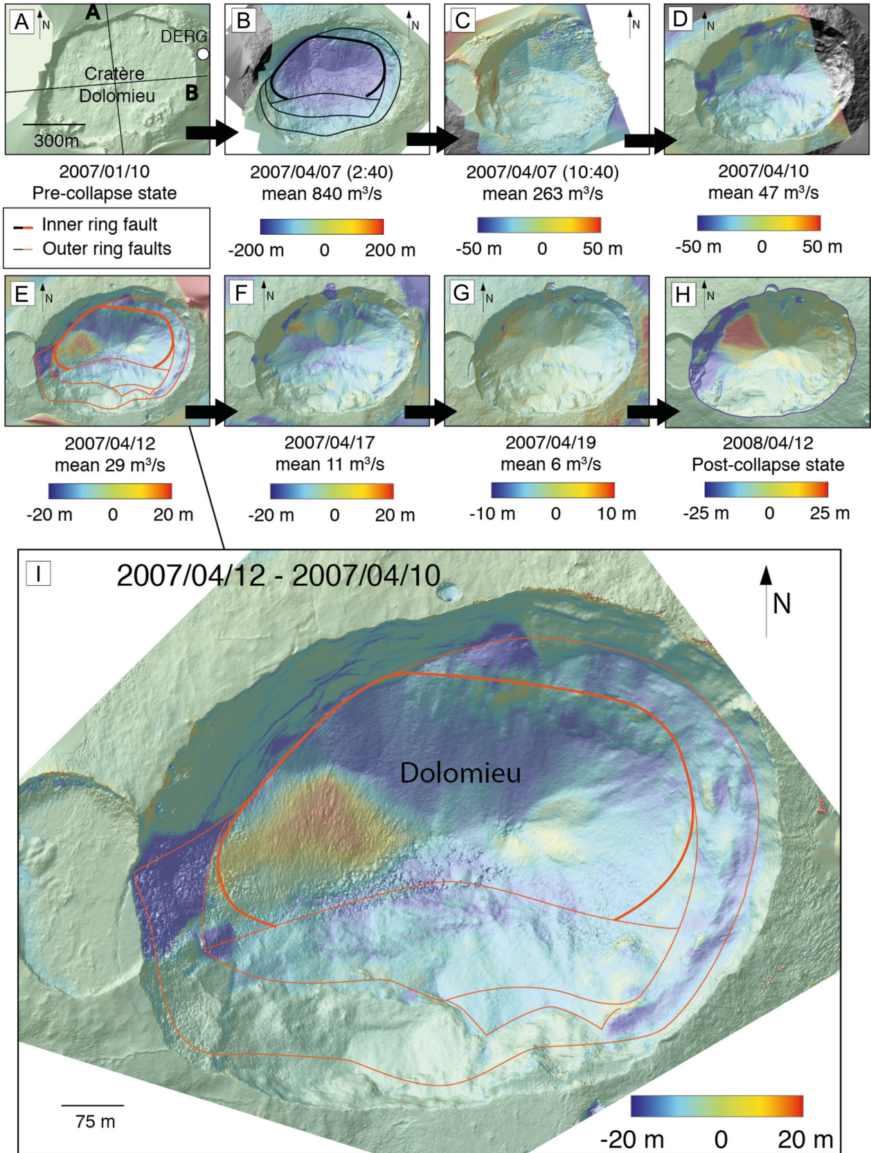
Figure 2: Evolution of subsidence inside the Cratère Dolomieu during and after the collapse, from vertical differences between consecutive DEMs. A and B on [A] are the locations of the cross-sections shown in Figure 3A, B. Rates are obtained by dividing the volume difference by the time period between two acquisitions. The thick and thin red contours on [E] and [I] are the outlines of the IRFs (Inner Ring Faults) and ORFs (Outer Ring Faults), respectively, reported in Figure 4B.
