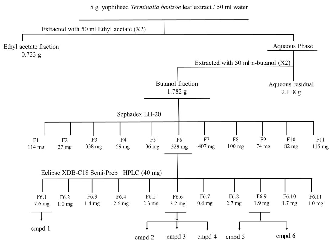
Figure 3. MTT-guided fractionation of T. bentzoe extract cytotoxicity against HepG2 cells. Compd: Compound. Compd 1 = \alpha and \beta - Punicalagin; compd 2 = Isoterchebulin; compd 3 = Terflavin A; compd 4 = 3,4,6-trigalloyl- \beta -D-glucopyranose; compd 5 = 2''-O-galloyl-orientin; compd 6 = 2''-O-galloyl-isoorientin.
