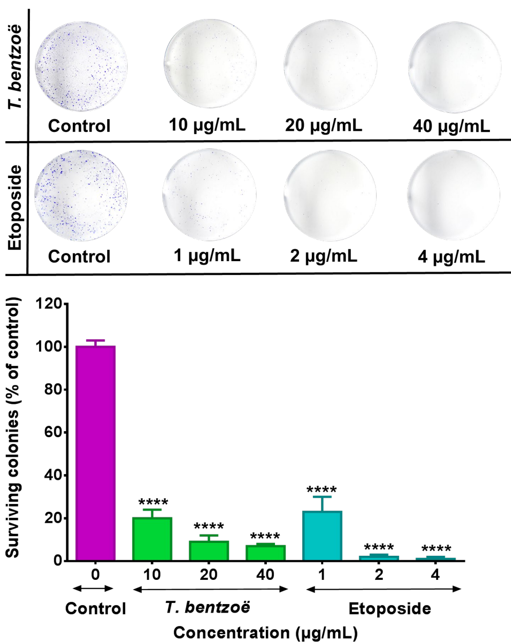
Figure 1. HepG2 cells were treated with the indicated concentrations ( \mu\text{g/mL} ) of test extracts for 48 h and subsequently allowed to grow into colonies for 14 days. After 14 days, the colonies were stained with 0.1% crystal violet and the images of the wells were captured using a digital camera. The colonies were counted using Image J software. Each experiment was performed three times. Asterisks represent significant differences between extract treatments and untreated control, **** p \leq 0.0001 .
