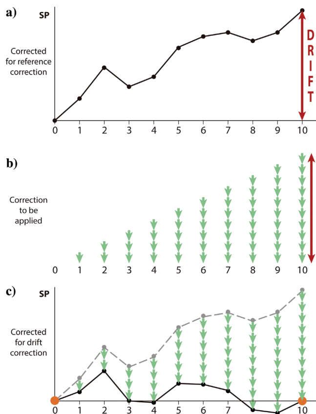
Figure 4. Schematic representation of (a) an SP profile composed of 10 measurements in which points 0 and 10 are either geographically the same or are linked by an isopotential line (e.g., sea, lake, or aquifer); the difference observed in the SP value is the drift. (b) The linear distribution of the drift from the reference (0 fractions of the drift) to point 10 (10 fractions of the drift, i.e., the total drift), in which one green arrow is one fraction of the total drift. (c) The application of the closure correction for the 10 data points, with points 0 and 10 now displaying the same SP value.
