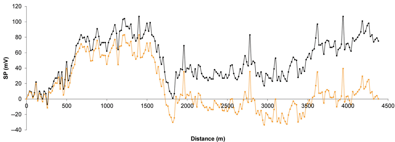
Figure 6. Example of the closure correction for an actual closed SP profile. The black line is the data set that has been previously corrected for the reference correction, and the orange line is the same data set after the application of the closure correction. The drift is exaggerated here, compared to the length of the profile, to get a perception of the effect of the closure correction. Note that the last point (at a 4380 m distance) is corrected to reach the same value as the reference point (at a 0 m distance; that is geographically the same point because it is a closed profile). Also note how this correction changes the SP values gradually without affecting the location of the SP maxima and minima.
