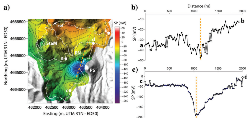
Figure 12. (a) Section of the SP map acquired in Garrotxa (Catalonia, Spain). (b and c) SP versus distance graphs along selected SP profiles (a b and c d). StaM, RN, and PS stand for the Santa Margarida, Rocanegra, and Puig Subià volcanoes, respectively, and ref is the reference for the SP data set. The dashed orange line is the eruptive fissure between RN and PS, and the small white dots are the SP measurements. Profile a b defines a real SP minimum, whereas c d shows a relative SP minimum (see the text for an explanation; [a and b] has been modified from Barde Cabusson et al., 2014).
