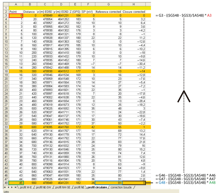
Figure 5. Closure correction of the SP data along one closed profile (or loop), using Excel. References are highlighted by the orange rows that mark the limits of each section of 300 m (the maximum length of the wire in this example). In column G, the first (cell G3) and the last (cell G48) SP measurements are at the same geographic location but they show different SP values (values after the reference correction). This difference (G48 - G3) corresponds to the drift of this profile. Column H shows the closure correction applied to correct for this drift. When applied to the whole loop, the first (cell H3) and the last (cell H48) display the same SP value (here, 0 mV). The $ sign is the formula that is used (in Excel) to keep the cell coordinates (the column letter and the row number) constant when the formula is copied through the rest of the column.
