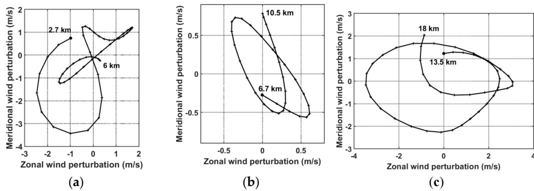
Figure 12. (a), (b) and (c) similar as Figure 11 but in the TC eye (23° N, 123.2° E).
