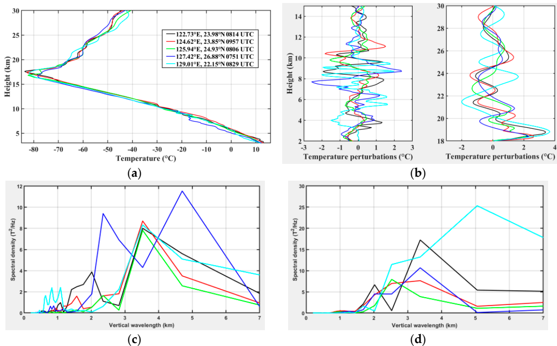
Figure 15. (a) FormoSat-3/COSMIC RO profiles of temperature at heights of 3–30 km from 07:51 UTC to 09:57 UTC nearby the TC on 7 August 2015. (b) Perturbations in the troposphere (left) at 2–15 km and LS at 18–30 km (right). Part (c) and (d) correspond to spectral density as a function of vertical wavelength respectively. For all figures, refer to colors in the legend of Figure 5a for the date and location of the RO profiles and also Figure 7a for the spatial distribution.
