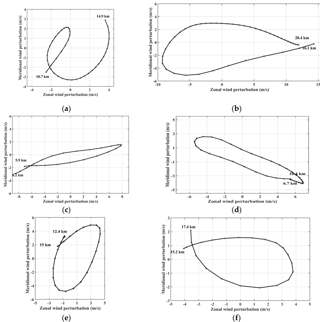
Figure 11. Hodographs of horizontal wind perturbations on 7 August 12:00 UTC. In the LS (a) at (23° N, 125° E) in the UT and (b) at (22° N, 126.4° E) in Region A; in the middle troposphere (c) at (23° N, 122° E) in Region B, (d) at (22° N, 124.9° E) in Region C; (e) at (25.5° N, 125.3° E) and (f) at (21° N, 128.8° E) in the UT in Region D respectively. Crosses visualize the vertical step of 100 m height. Regions A, B, C and D are drawn on the Figure 8.
