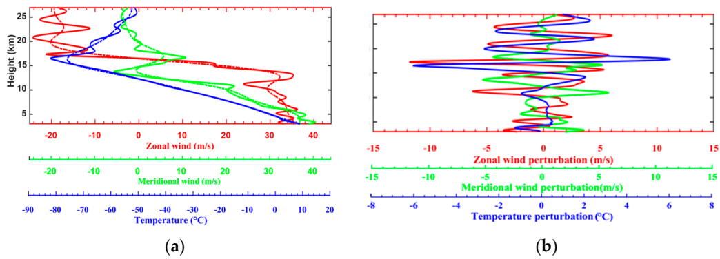
Figure 10. (a) Vertical profiles of zonal (solid red) and meridional wind (solid green), and temperature (solid blue) at location (22° N, 124.3° E) in region C. Mean vertical profiles (dash-dotted) are retrieved using a fourth-order Butterworth low-pass filter with a 7 km wavelength cutoff. (b) Temperature and horizontal wind perturbations.
