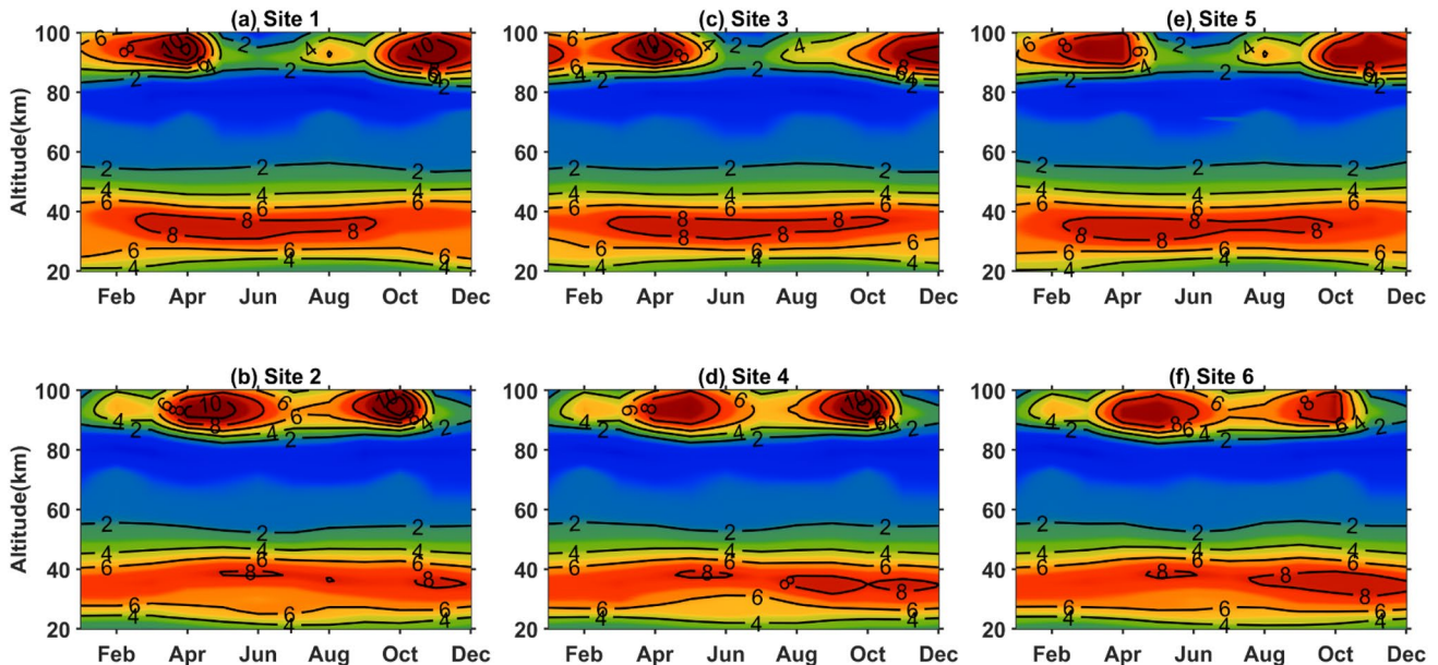
Fig. 2 Contour plots of climatological (2002–2015) ozone volume mixing ratio in parts per million (ppm) derived from SABER observations in the NH over a Site 1 ( 50^{\circ} N, 120^{\circ} W), b Site 3 ( 50^{\circ} N, 2.5^{\circ}
