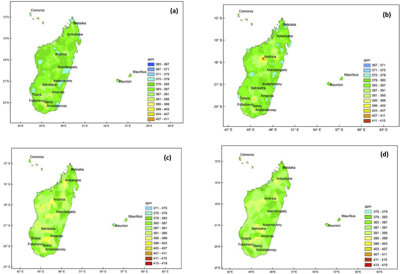
Fig. 3. Seasonal CO 2 surface spatial distribution over the SWIO islands: Fig. 3a to d illustrate spatial distribution during the austral summer (DJF), autumn (MAM), winter (JJA) and spring (SON), respectively.
