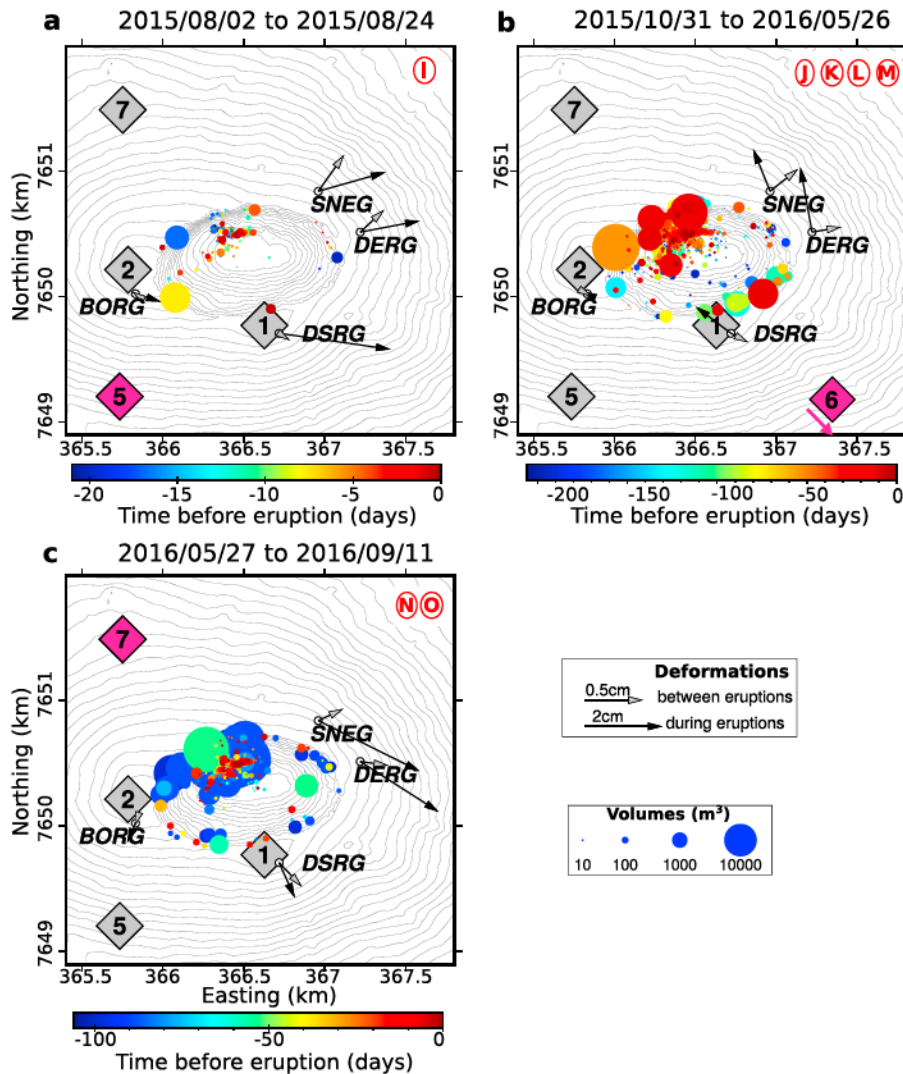
Figure 13. Same as Figure 12 for eruptions 5 to 7. (a) Eruption 5: 24 August to 31 October 2015, (b) Eruption 6: 26 and 27 May 2016, and (c) Eruption 7: 11–18 September 2016.
