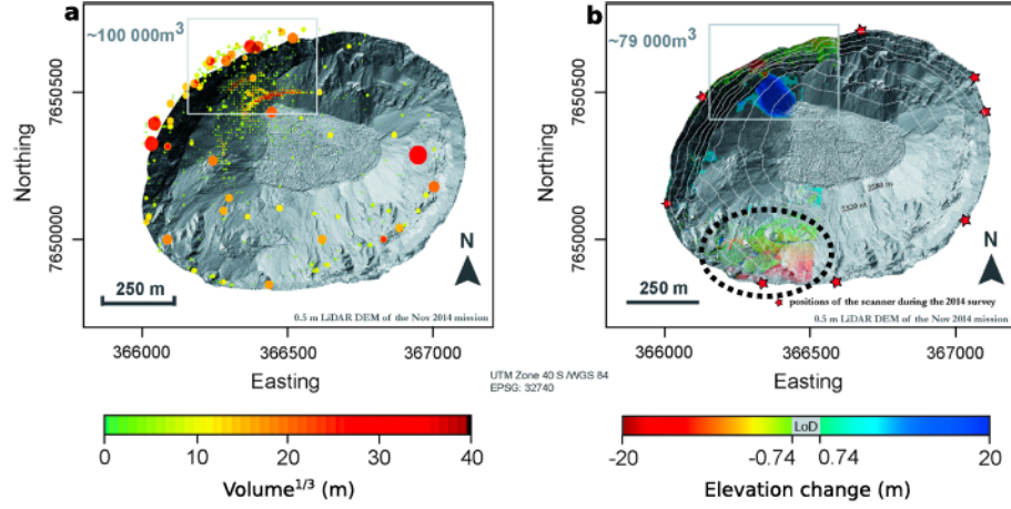
Figure 3. (a) Volumes of the RFs ( V^{1/3} is represented) that occurred from October 2014 to January 2016, computed using seismic signals. Each round dot represents a RF, and its radius and color are proportional to the cubic root of the RF volume. The white square defines the area where the total volume ( 100,000 \text{ m}^3 ) is computed. (b) Same as (a) but using photogrammetric data and method. The dotted ellipse highlights the inferred subsiding zone. RF = rockfall.
