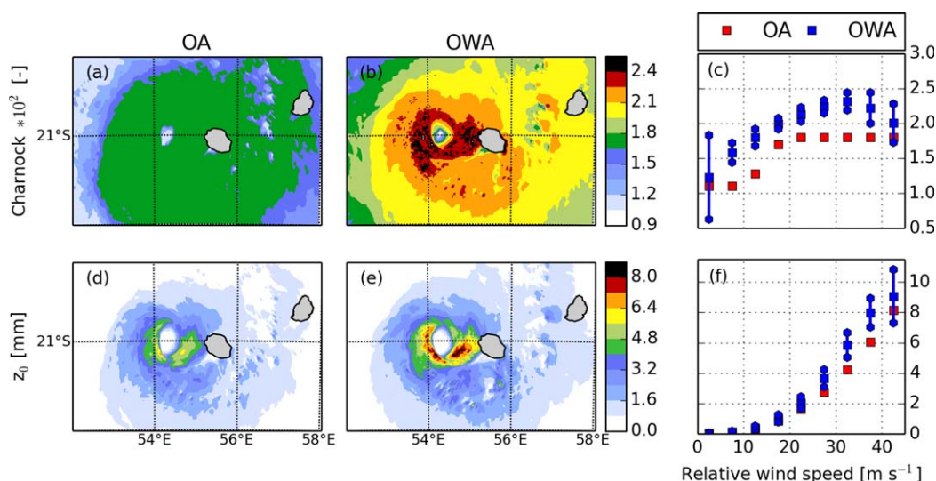
Figure 10. (left plots) Charnock parameter (w/o unit; first row) and roughness length (mm; second row) at 06 UTC on 2 January 2014 for the OA and (middle plots) OWA simulations. (right plots) Scatterplot of the Charnock parameter and roughness length versus relative wind speed. Blue and red squares correspond to mean values and blue diamonds correspond to the standard deviation.
