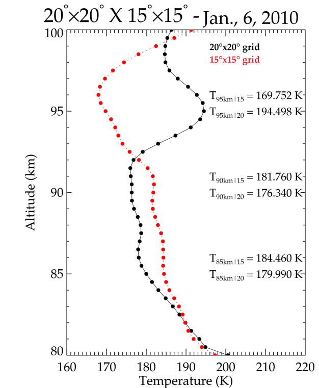
Figure 3. Temperature profiles of the MLT region as retrieved from SABER/TIMED observations over Santa Maria, southern Brazil, on 6 January 2010. The 20^\circ \times 20^\circ lat/long grid profile is shown in black, while the 15^\circ \times 15^\circ profile is shown in red.
