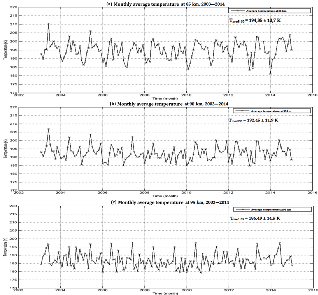
Figure 5. Monthly average temperature values at 85 (a), 90 (b) and 95 (c) km height derived within a \pm 7.5^\circ grid over Santa Maria, for the 2003–2014 period.
