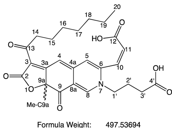
Fig. 4. Molecular structure and carbon atom numbering of compound n. 4. Proposed Name: N-GABA-PP-V, 4- \{6-[(E)-2\text{-Carboxyvinyl}]-9\text{-methyl-3-octanoyl-2,9-dioxo-9,9a-dihydrofuro}[3,2-g]\text{isoquinolin-7(2H)-yl}\} butanoic acid.
