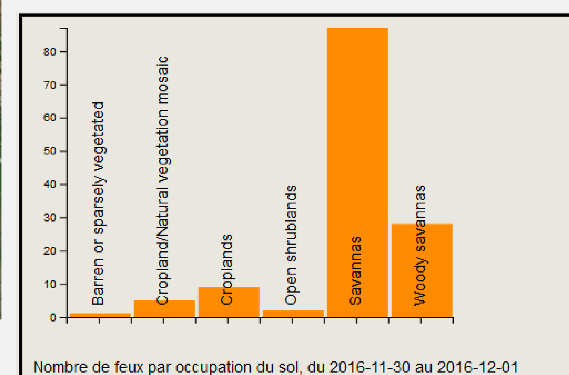
Statistics on land-use patterns affected by fires between 30 November and 01 December 2016. According to the Global Land Cover 2012 classification. Example of statistics extracted automatically from the online interface.
