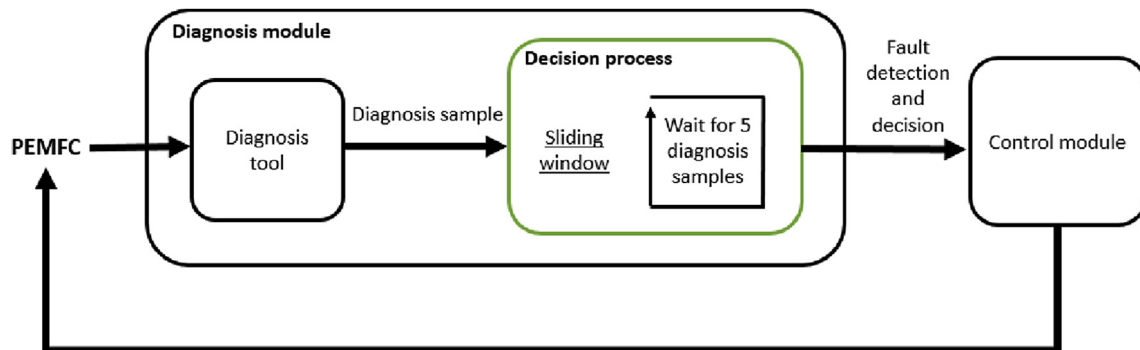
Fig. 4. Decision process based on a sliding window.
