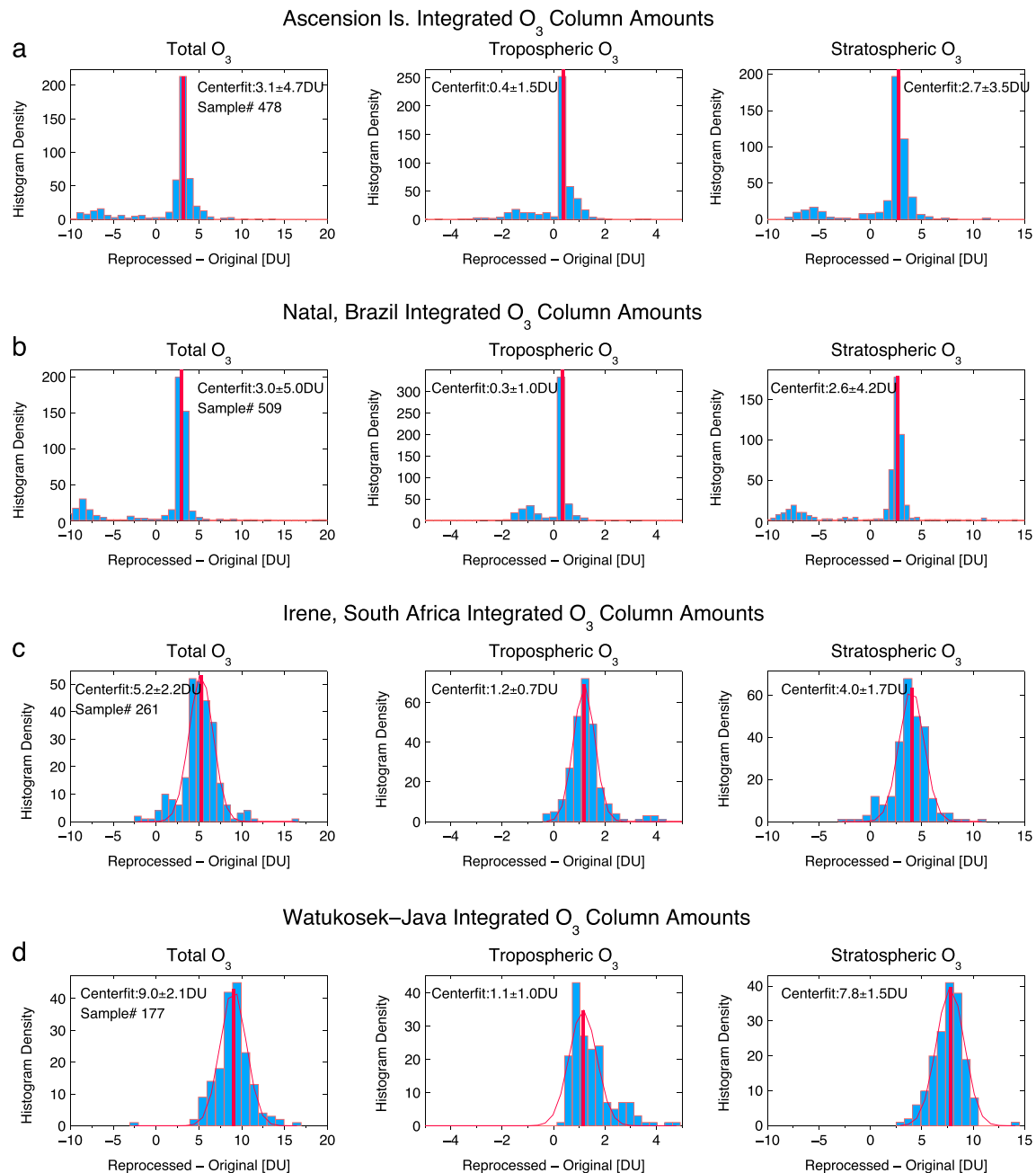
Figure 3. (a–g) Histograms of the difference between the reprocessed and original profiles per site. Total integrated (ICO total ) (left), tropospheric (middle), and stratospheric (right) O 3 columns are shown. ICO total amounts are integrated up to 5 hPa with a 15 hPa balloon burst limit. (c–f) Red curves in Figures 3c–3f are the Gaussian fit to the histograms that do not exhibit bimodal behavior. Red vertical lines indicate the centerfits of the distribution. Data gaps and pressure bursts at altitudes below 15 hPa have led to sample size reductions of Figure 3a, 14% at Ascension; Figure 3b, 7% at Natal; Figure 3c, 15% at Irene; Figure 3d, 30% at Watakosek; Figure 3e, 36% at Kuala Lumpur; Figure 3f, 15% at La Réunion; and Figure 3g, 24% at Hanoi.
