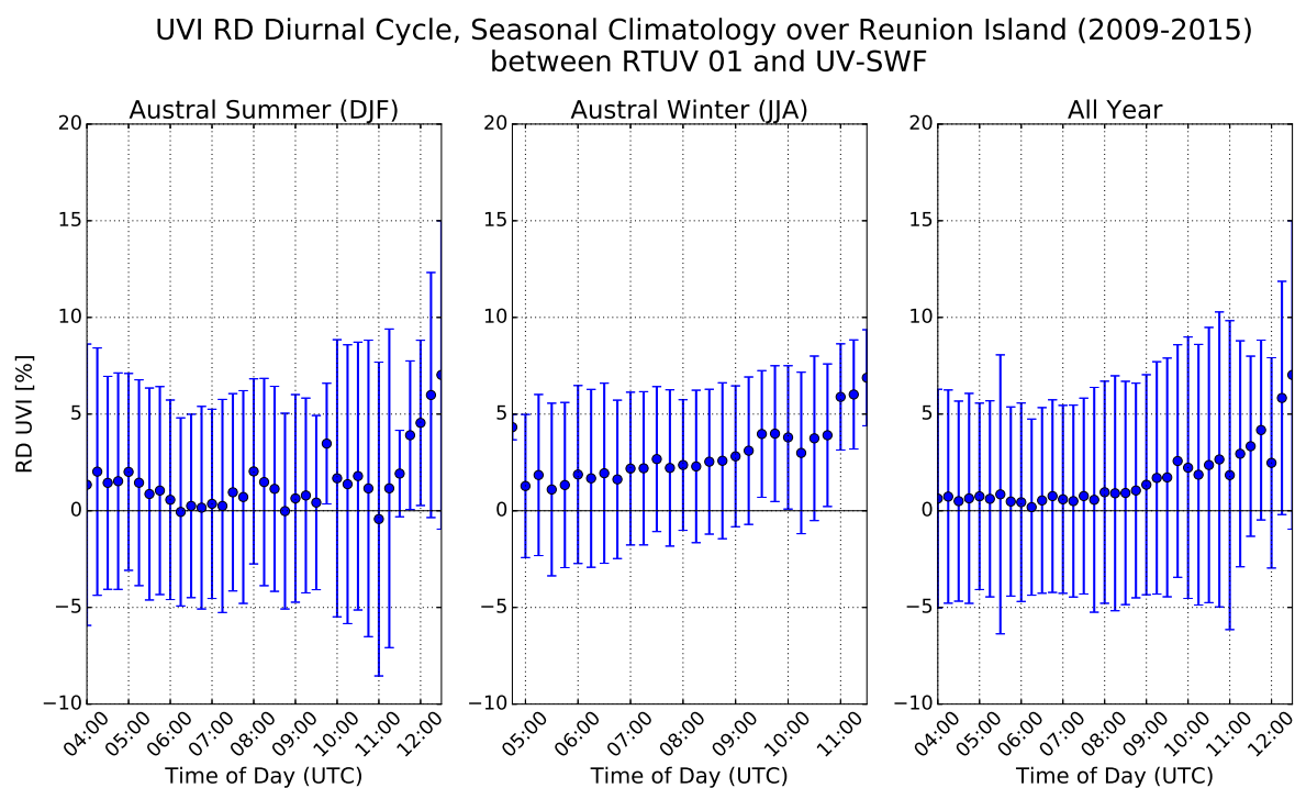
Figure 10. Diurnal Cycle of UVI Relative Difference between RTUV01 and UV-SWF for Austral Winter, Summer, and All Year. UVI relative differences every 15 minutes are in blue dots with dispersion bar ( \pm 1 \sigma (standard deviation)).
