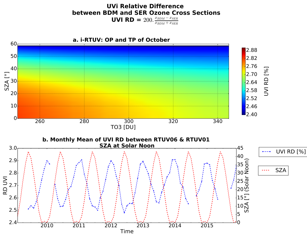
Figure 5. a) UVI Relative Difference between two idealized runs with different O3XS for a varying TO3 and SZA and for climatological OP and TP of October. b) Monthly Mean of UVI RD between RTUV06 and RTUV01 (blue dashed line). Monthly Mean of SZA at Solar Noon. (red dashed line)
