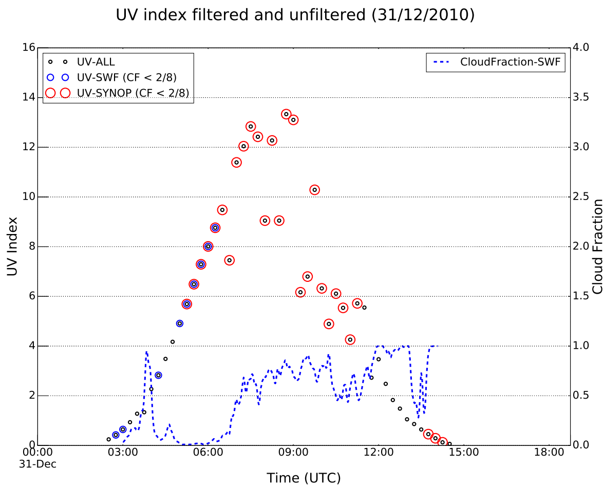
Figure 1. Daily UV index at La Réunion on December 31, 2010; for UV-all Bentham measurements in black circles, UV-SWF: UV data filtered with CF-SWF in blue circles, UV-SYNOP: UV data filtered with CF-SYNOP in red circles. Cloud Fraction (CF-SWF) is also represented by the blue dashed line.
