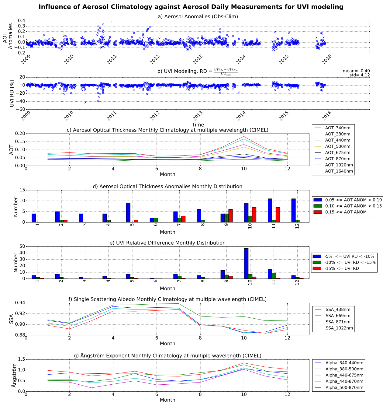
Figure 7. Impact of aerosols on UVI modelling.
