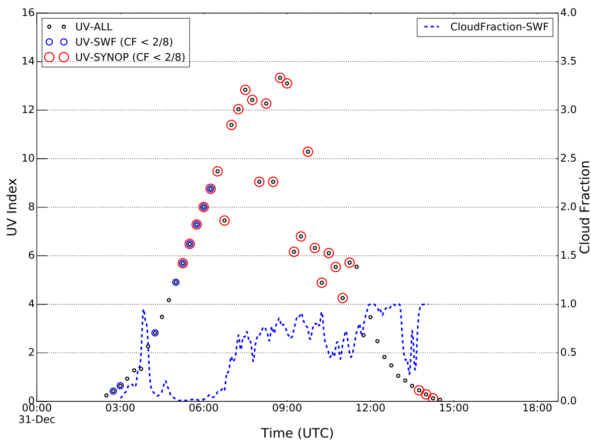
Figure 1. Daily UV index at La Réunion on December 31, 2010; for UV-all Bentham measurements in black circles, UV-SWF: UV data filtered with CF-SWF in blue circles, UV-SYNOP: UV data filtered with CF-SYNOP in red circles. Cloud Fraction (CF-SWF) is also represented by the blue dashed line.
