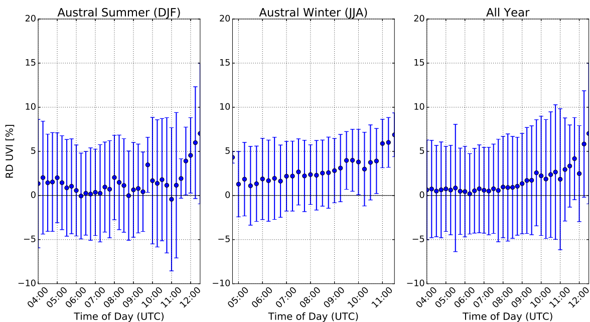
UVI RD Diurnal Cycle, Seasonal Climatology over Reunion Island (2009-2015) between RTUV 01 and UV-SWF
