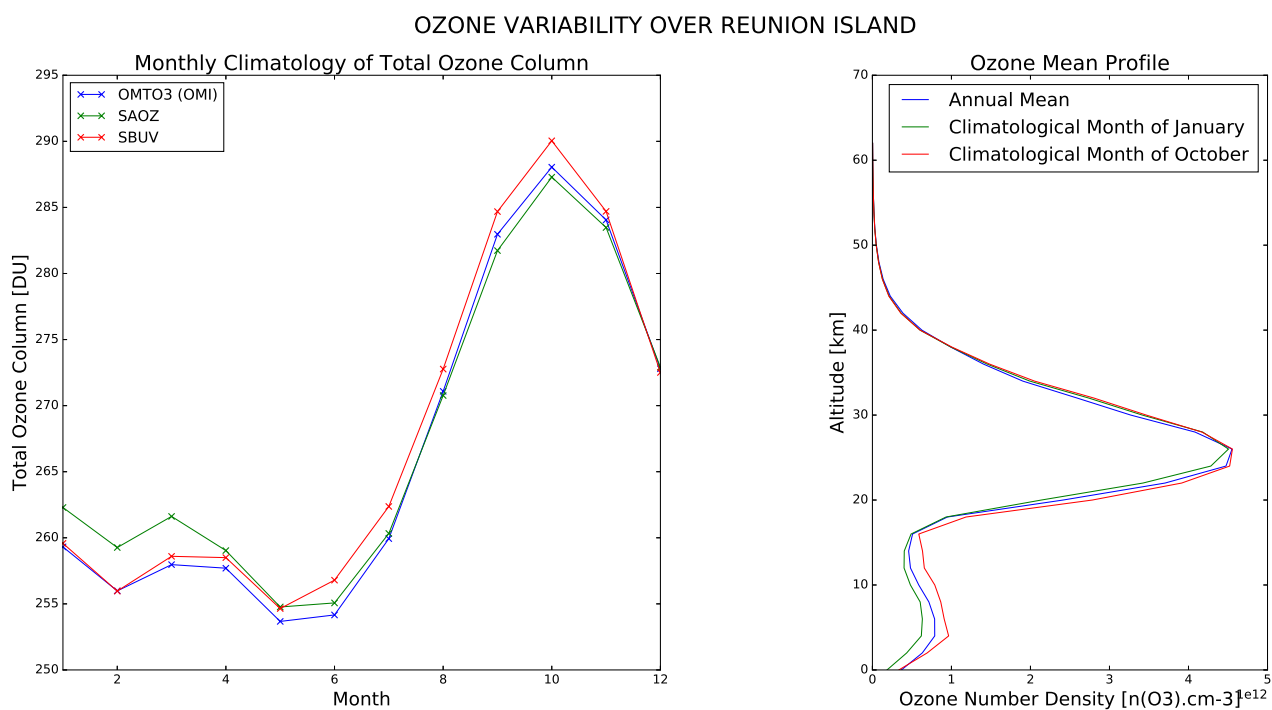
Figure 3. Ozone Variability over Reunion Island. Left : Monthly Climatology of Total Ozone Column for three datasets (OMI in blue, SAOZ in green and SBUV in red) Right: Mean Ozone Profile from McPeters and Labow [2012] Climatology. Annual mean in blue, January in green and October in red.
