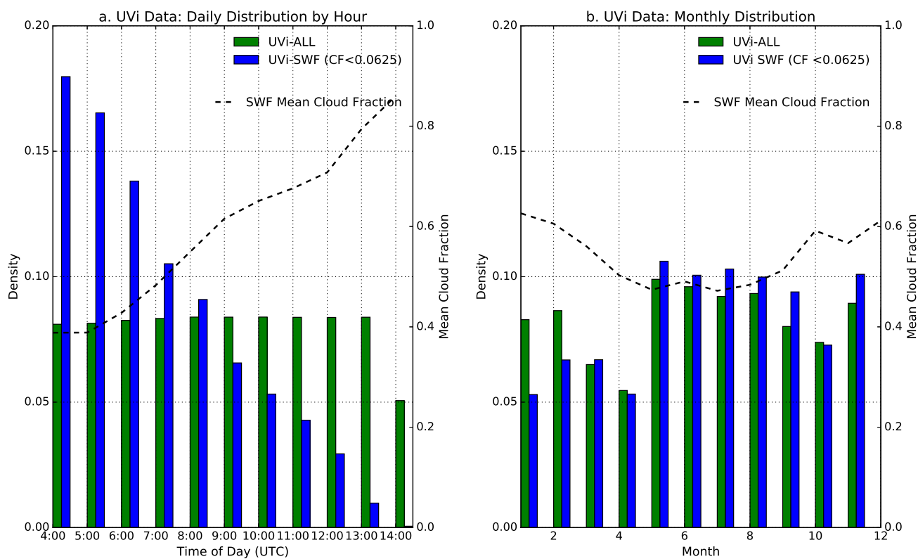
Figure 2. UVI data distribution and Cloud Fraction for 1h bins. UVI-all in green, UVI-SWF in blue, Cloud Fraction in dotted line.
