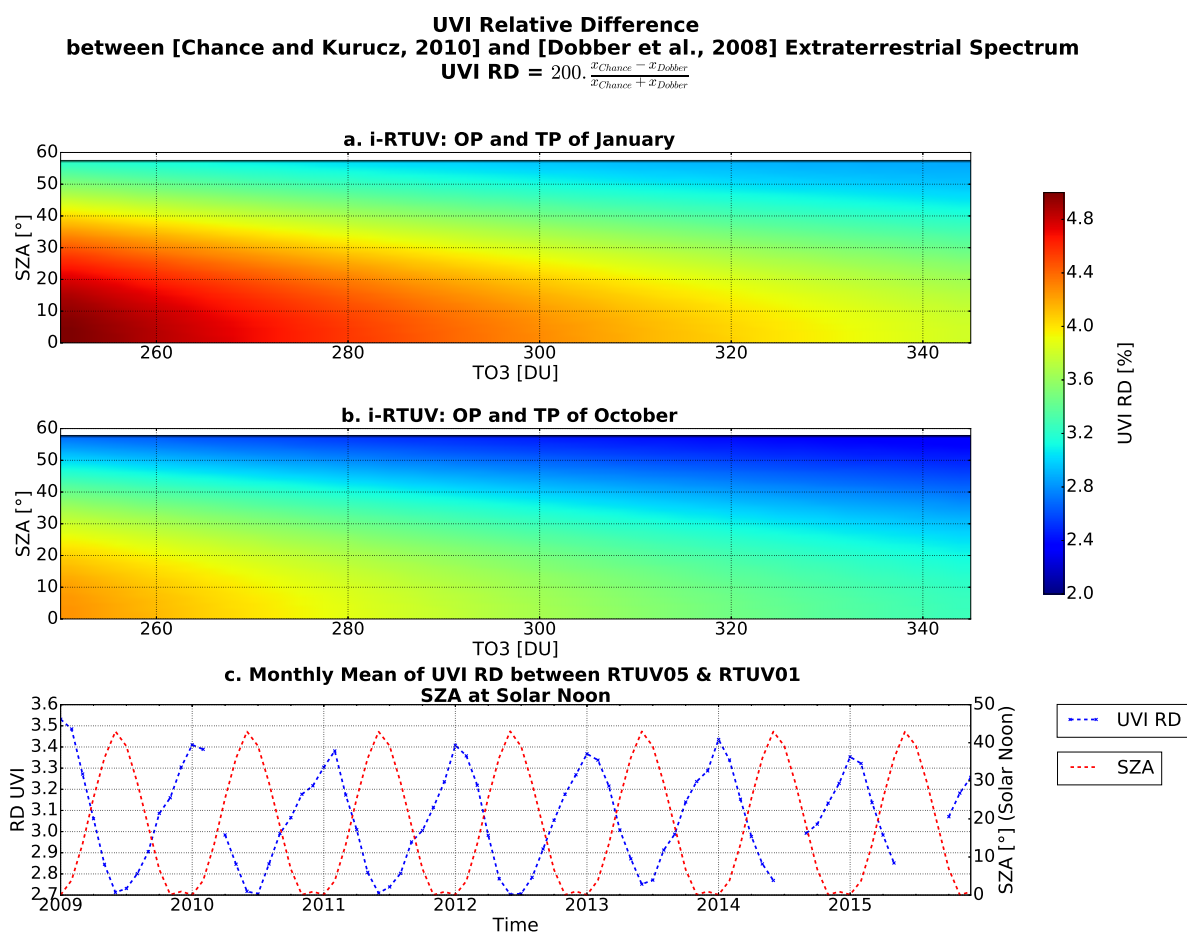
Figure 4. a) UVI Relative Difference between two idealized runs with different ET spectra for a varying TO3 and SZA for a climatological OP and TP of January b) Same as a) but for OP and TP of October. c) Monthly Mean of UVI RD between RTUV05 and RTUV01 (blue dashed line). Monthly Mean of SZA at Solar Noon. (red dashed line)
