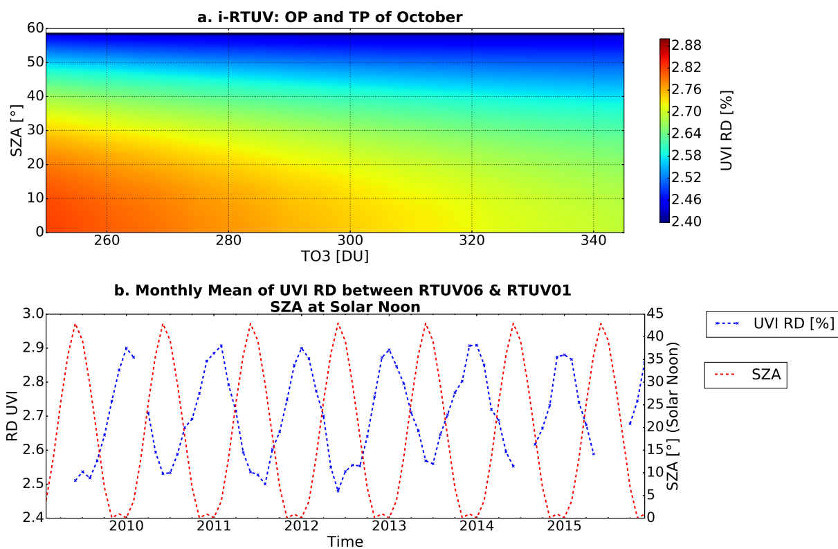
Figure 5. a) UVI Relative Difference between two idealized runs with different O3XS for a varying TO3 and SAZ and for climatological OP and TP of October. b) Monthly Mean of UVI RD between RTUV06 and RTUV01 (blue dashed line). Monthly Mean of SAZ at Solar Noon. (red dashed line)
