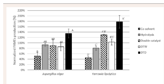
Figure 4 Plot of the normalized FAMES production from wet biomass and dry biomass, by different esterification procedures, for A. niger and Y. lipolytica . Normalised FAMES production (%) was calculated as percentage of the FAMES production by the Reference two-step method of choice, for each microorganism. A-C represent significantly different classes for A. niger biomass. A'-D' represent significantly different classes for Y. lipolytica biomass.
