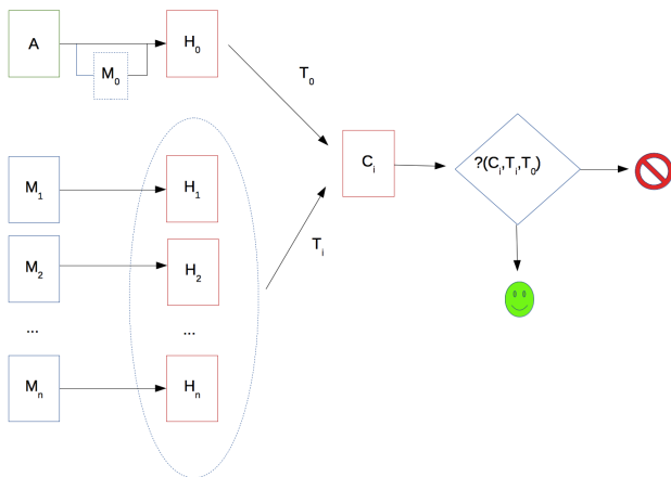
Figure 2. The algorithm recognition process.
