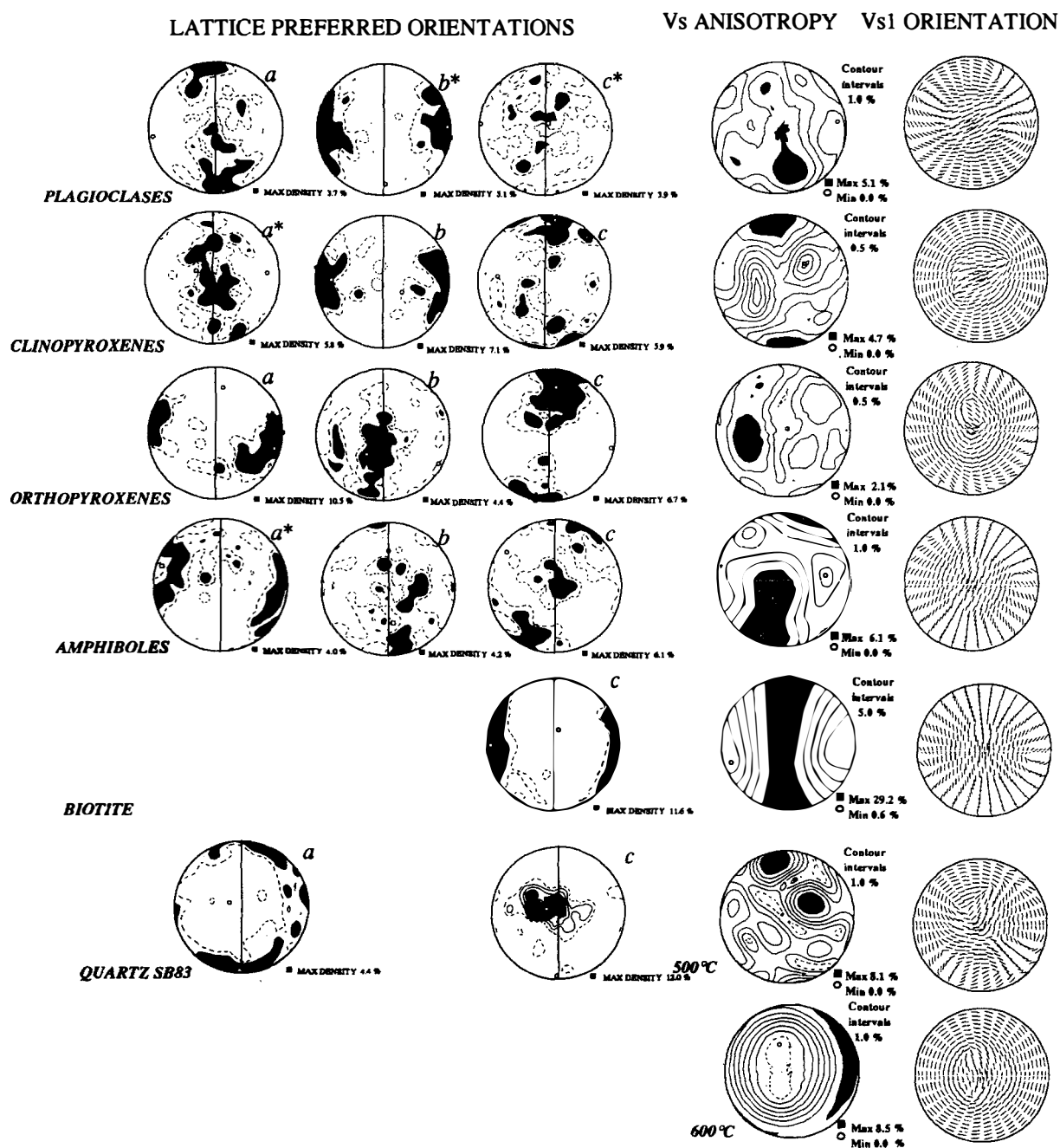
Fig. 6. Typical LPO of the main crystallographic axes of crustal mineral phases selected to model S-wave properties of synthetic crustal rocks. The projections are in the structural reference frame: foliation is north-south and lineation is north-south. Maximum density of crystallographic axes is marked by a filled square (left). The 3-D variations of the birefringence anisotropy of the ideal aggregate composed of 100% of the given mineral with the measured LPO and the fast split shear-wave polarization plane orientations are shown on the right. For more details see text.
