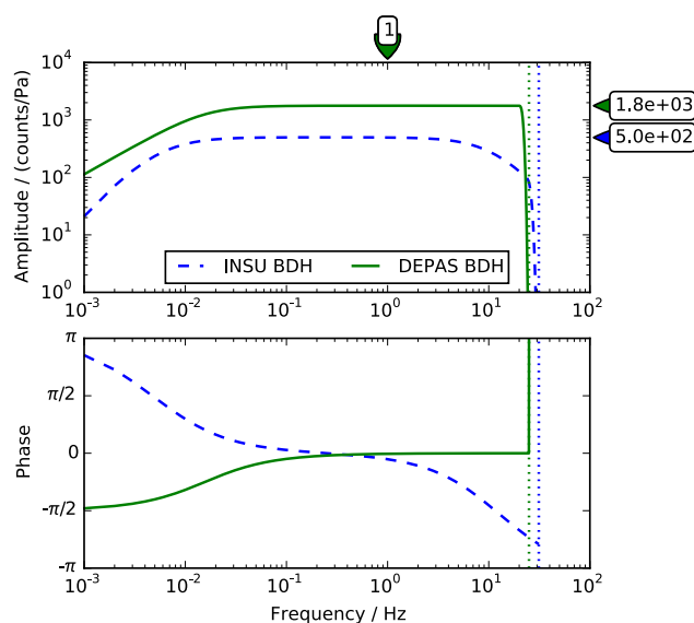
Figure 5. Bode plot of the total instrument responses G(f) as defined in Eq. (A2) of a DEPAS HighTechInc HTI-PCA04/ULF hydrophone (solid green, station RR26), and of an INSU differential pressure gauge (dashed blue, RR28). The nominal corner period is 100 s for DEPAS instruments and 500 s for INSU instruments. Dotted lines mark the Nyquist frequencies (see above).
