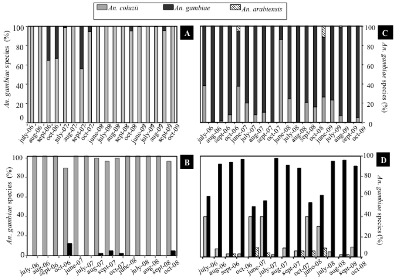
Fig. 5. Proportion of M and S forms of Anopheles gambiae and Anopheles arabiensis males sampled from swarms (A) and females collected indoors (B) in Vallée du Kou (VK7) and respectively in Soumouso (C-D).
