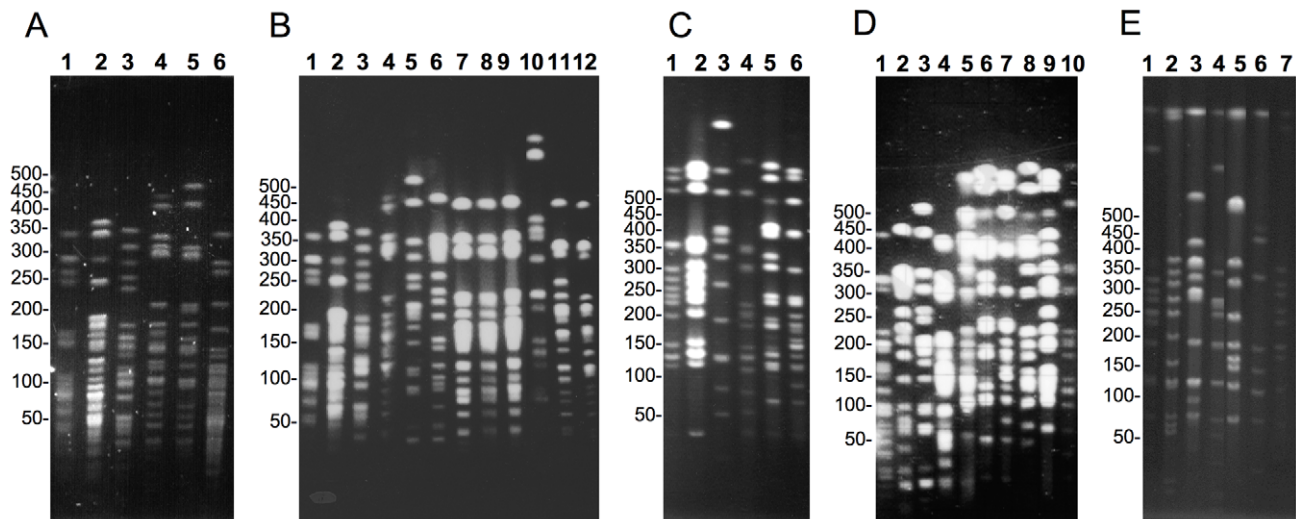
Figure 4. PFGE separation of NotI -digested genomic DNA from Leptospira isolates. A. Reference strains from serogroup Mini: serovars Beye (1), Georgia (2), Rugarupae (3), Mini (4), Swajizak (5), and Tbaquite (6). B. serovar Beye (1), serovar Georgia (2), serovar Rugarupae (3), serovar Mini (4), 2008/01927 (5), 2008/01929 (6), 2008/01931 (7), 2008/02842 (8), 2008/01924 (9), serovar Kambale (10), serovar Nona (11), and serovar Jules (12). C. serovar Grippotyphosa strain Valbuzzi (1), serovar Grippotyphosa strain Moskva V (2), serovar Grippotyphosa strain Andaman (3), 2008/01774 (4), 2008/03703 (5), 2008/00695 (6). D. serovar Jules (1), 2008/01773 (2), 2008/01927 (3), 2008/01926 (4), 2008/02843 (5), 2008/03703 (6), 2008/00695 (7), 2008/01925 (8), 2008/02841 (9), 2008/01774 (10). E. 2007/01872 (1), serovar Abramis (2), serovar Biggis (3), serovar Camlo (4), serovar Guaratuba (5), serovar Manilae (6), and serovar Pyrogenes (7). The molecular weight size marker consisted of bacteriophage lambda DNA concatemers of 50 kb. doi:10.1371/journal.pntd.0000724.g004
