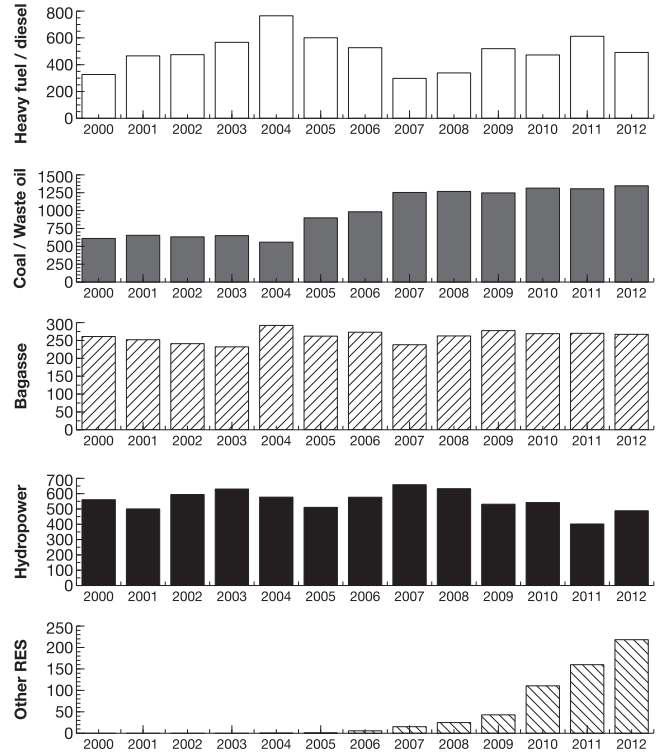
Fig. 3. Electricity mix [GW h] of Reunion since 2000.
