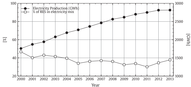
Fig. 4. Reunion self-sufficiency rate in electricity from 2000 to 2012.
