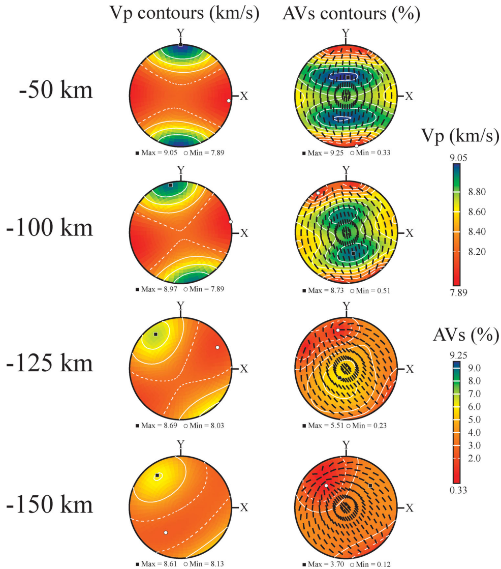
Figure 6. Lower hemisphere stereoplots in the thermomechanical reference frame (+ X to the right, + Y to the top and + Z vertical upwards) presenting the seismic properties (calculated for 70 per cent olivine–30 per cent enstatite aggregates) of domains localized at different depths (50, 100, 125 and 150 km from top to bottom) beneath the fault zone.
