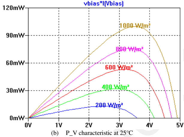
Figure6. Effect of varying ambient radiation (at 25°C)
