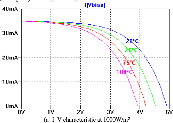
(a) I_V characteristic at 1000W/m²
