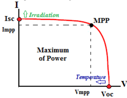
Figure3. Current-Voltage (I-V) characteristic for the PV cell
