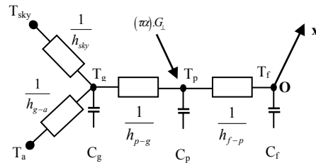
Figure 2 Thermal networks for the 3-node model.
