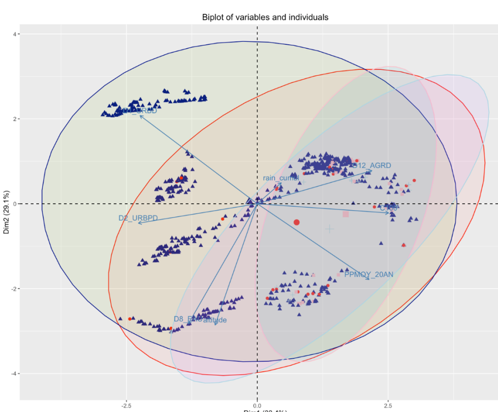
PCA of the landscape metrics to discern rodents by positivity and species (in Mahe, Seychelles)
